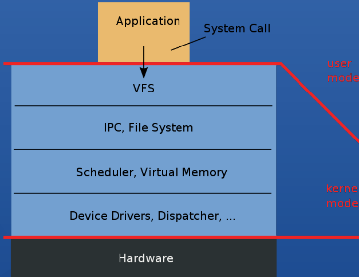
Monolithic Kernel based Operating System
